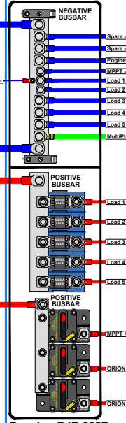
Drawing BJE-285B
